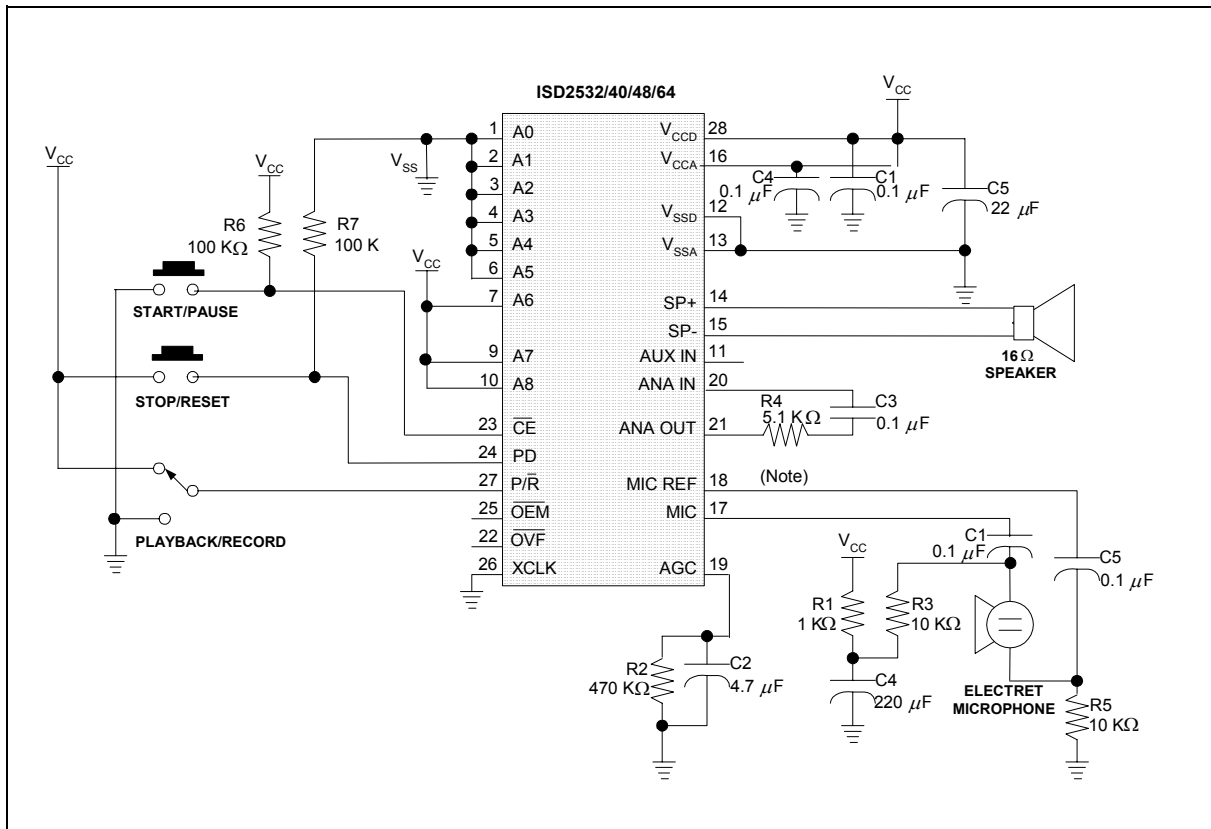
FIGURE 7: ISD2532/40/48/64 APPLICATION EXAMPLE – PUSH-BUTTON
